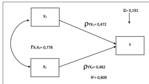
Figure 1. Path Analysis
